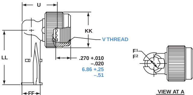
90 DEGREE ELBOW STYLE *10-630935-XXX
