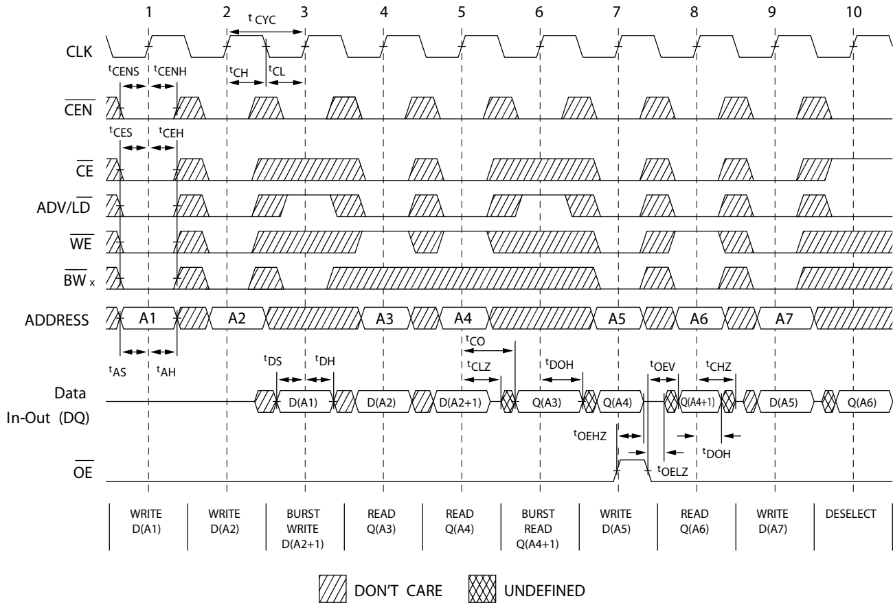
Figure 6. Read/Write Timing
