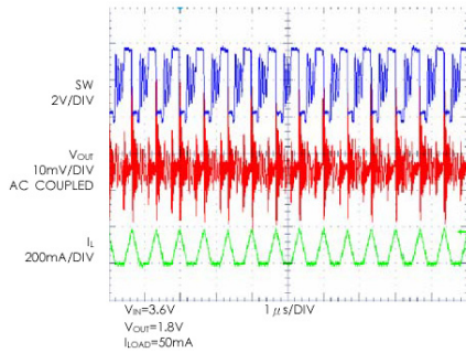
Fig. 14: Discontinuous Operation
