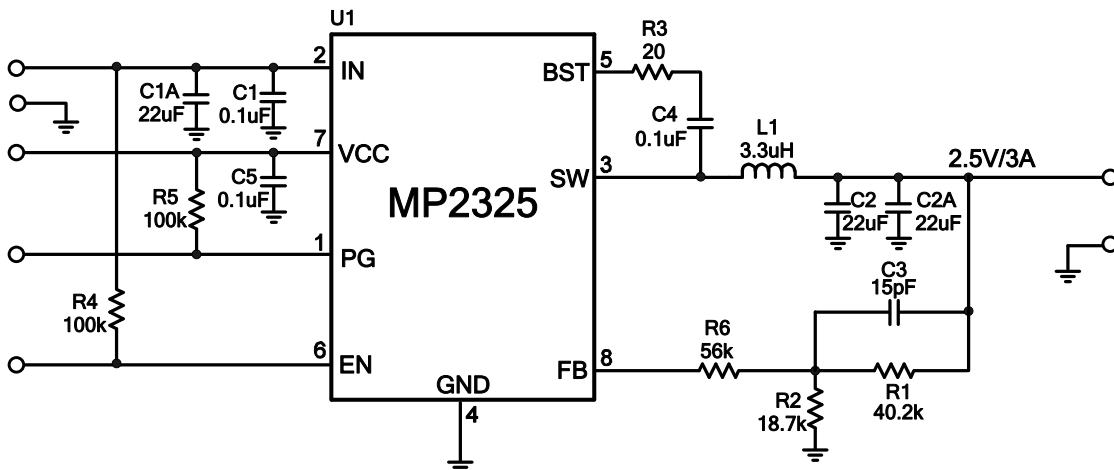
Figure 10: V_o=2.5V , I_o=3A
