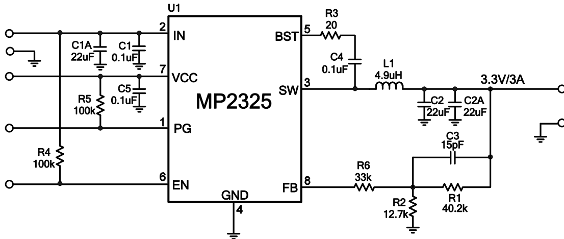
Figure 9: V_o=3.3V , I_o=3A
