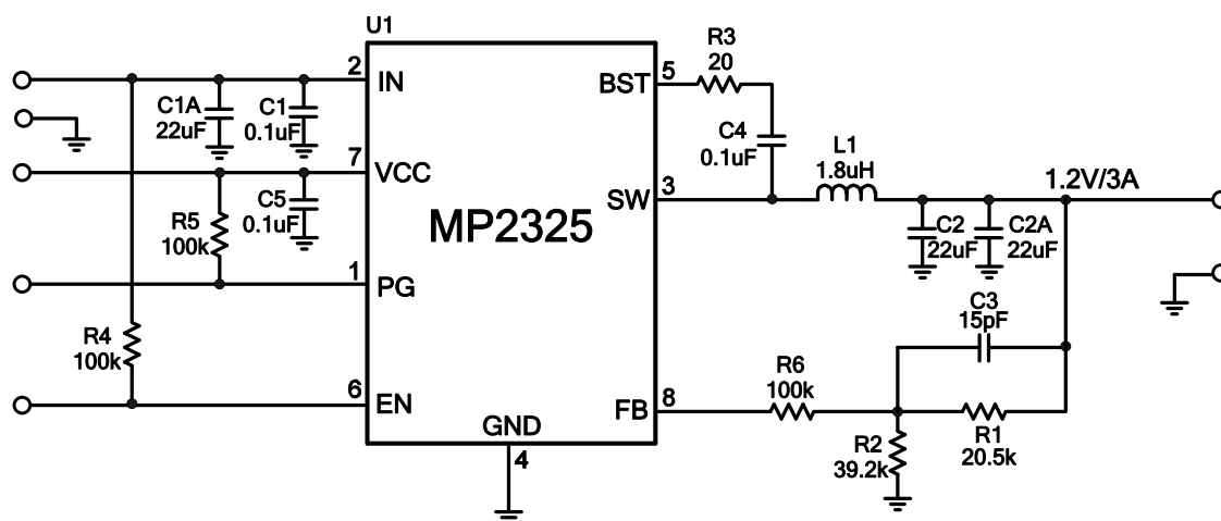
Figure 12: V_o=1.2V , I_o=3A
