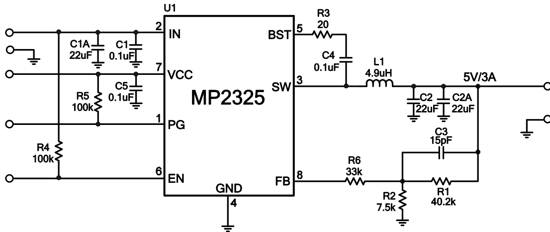
Figure 8: V_o=5V , I_o=3A
