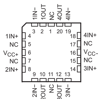
TL064 ... FK PACKAGE (TOP VIEW)
