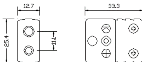
Standard Plug
