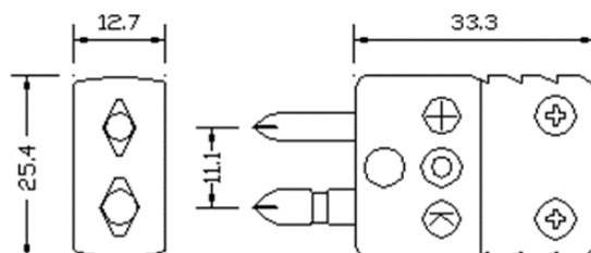
Standard Connectors:
