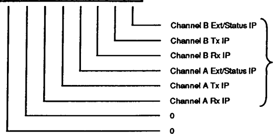
Read Register 3
