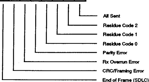
Read Register 1
