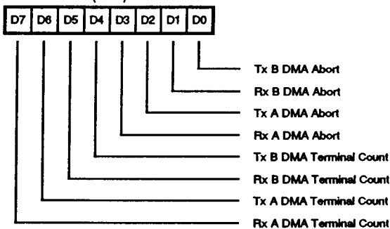
Address: 00000 (Read)
