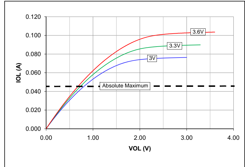
FIGURE 27-6: V_{OL} – 16x DRIVER PINS
