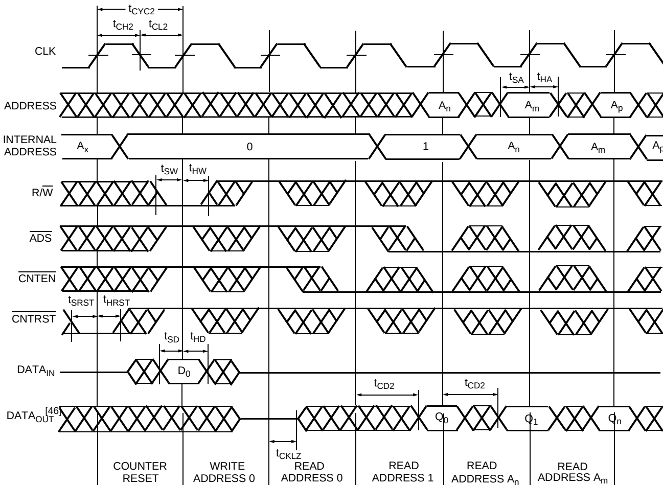
Figure 19. Counter Reset [44, 45, 46]
