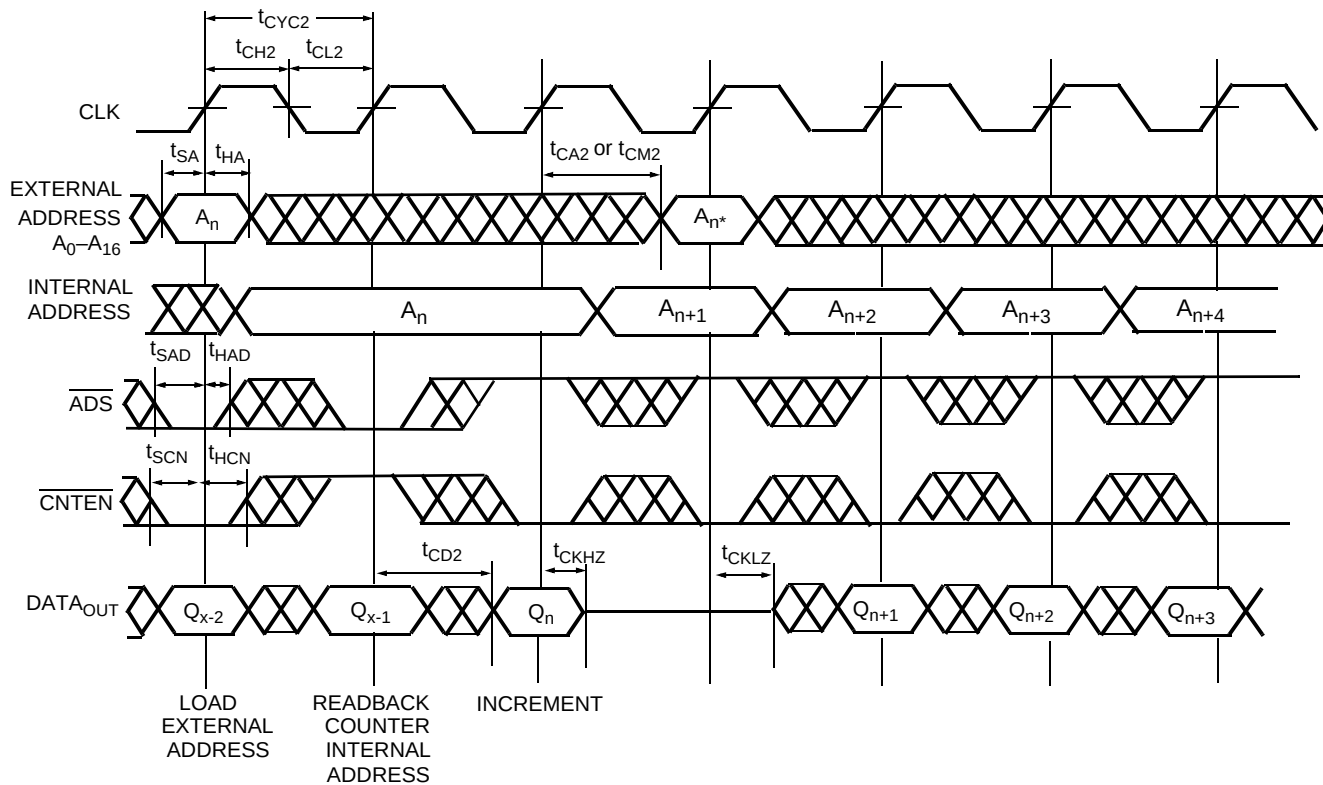
Figure 20. Readback State of Address Counter or Mask Register [47, 48, 49, 50]
