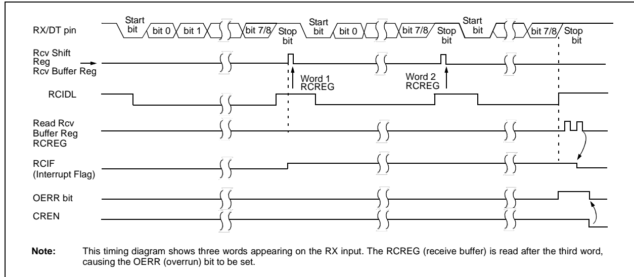
FIGURE 18-5: ASYNCHRONOUS RECEPTION
