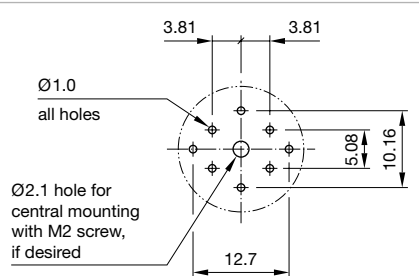
Component layout 1
