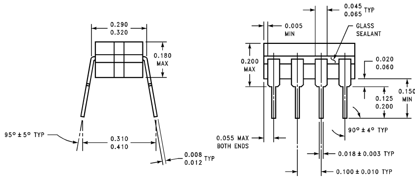
Cerdip Package (J) NS Package Number J08A
