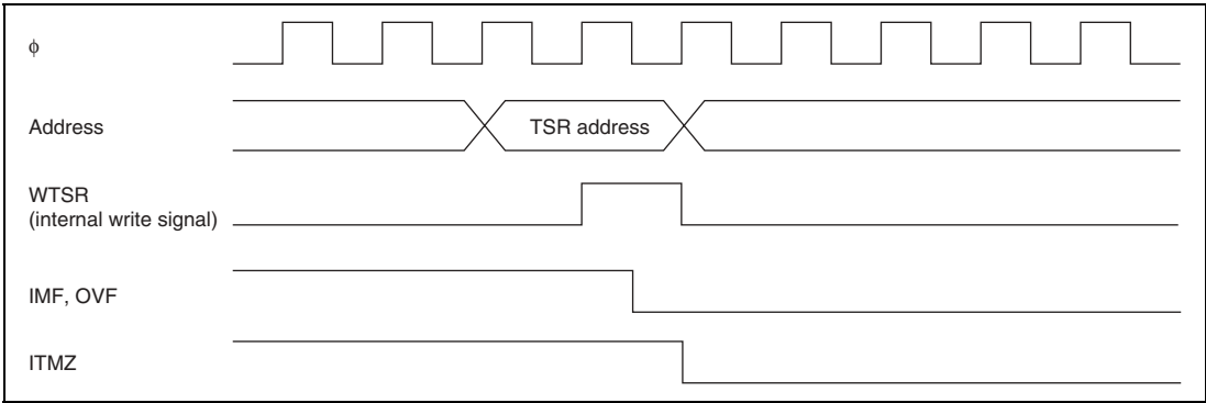
Figure 13.51 Status Flag Clearing Timing
