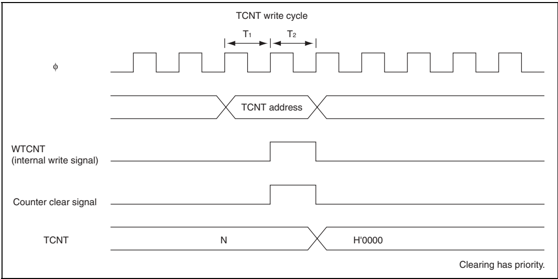
Figure 13.52 Contention between TCNT Write and Clear Operations
