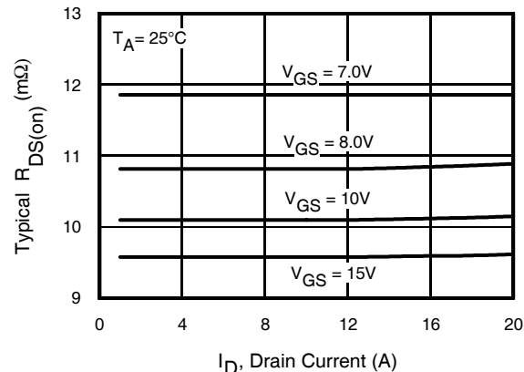
Fig 2. Typical On-Resistance Vs. Drain Current
