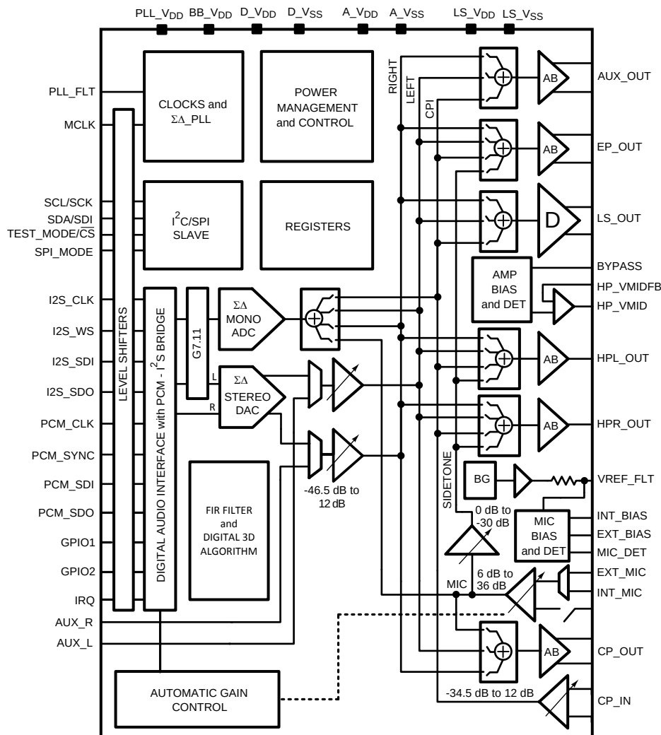
Figure 1. Conceptual Schematic
