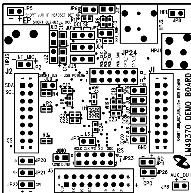
Figure 220. Top Silkscreen
