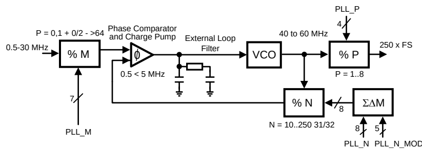
Figure 14. PLL Overview
