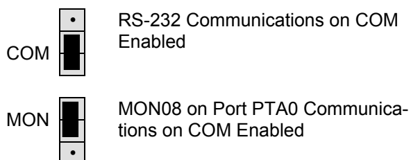
Figure 4: COM_MODE Jumper
