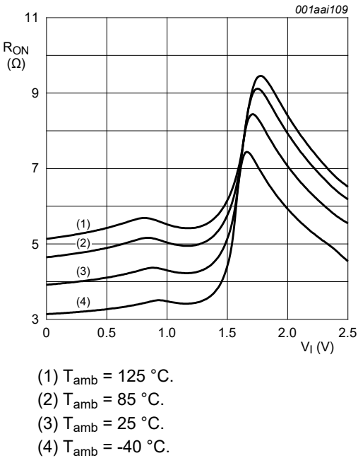
Fig. 6. ON resistance as a function of input voltage; V_{CC} = 2.5\text{ V} ; I_{SW} = 15\text{ mA}
