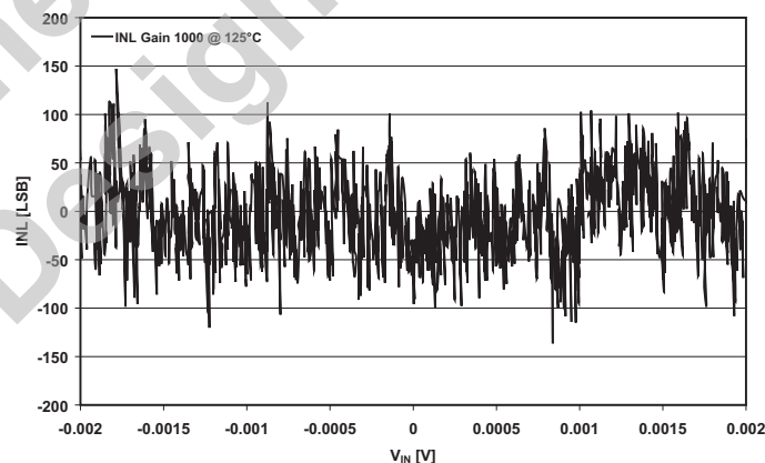
Figure 44. INL 125°C
