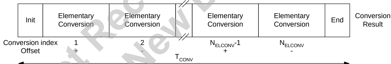
Figure 14. Analog-to-Digital Conversion Sequence
