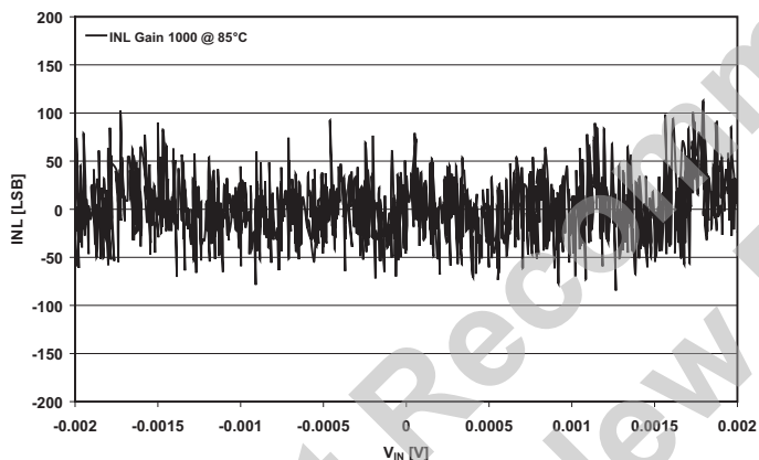
Figure 43. INL 85°C
