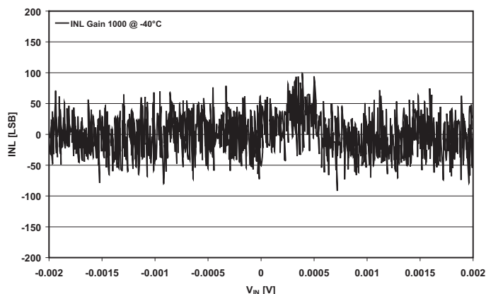
Figure 41. INL -40°C
