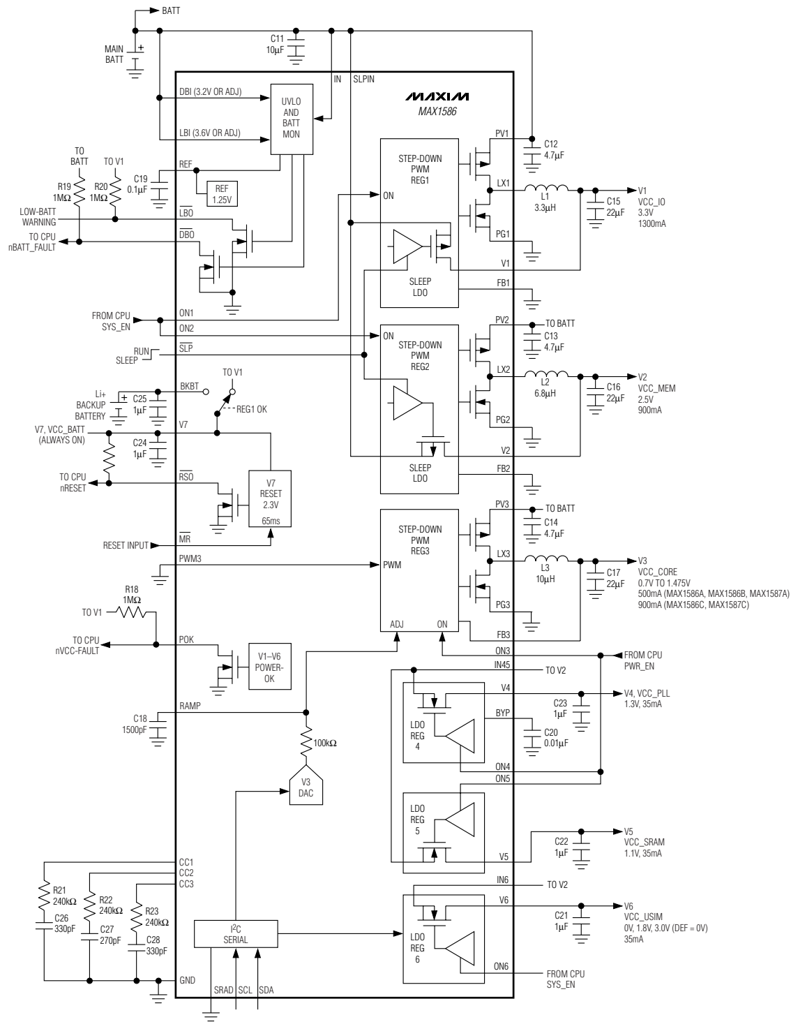
Figure 6. MAX1586 Typical Applications Circuit (The MAX1587 omits some features. See the Pin Description section.)
