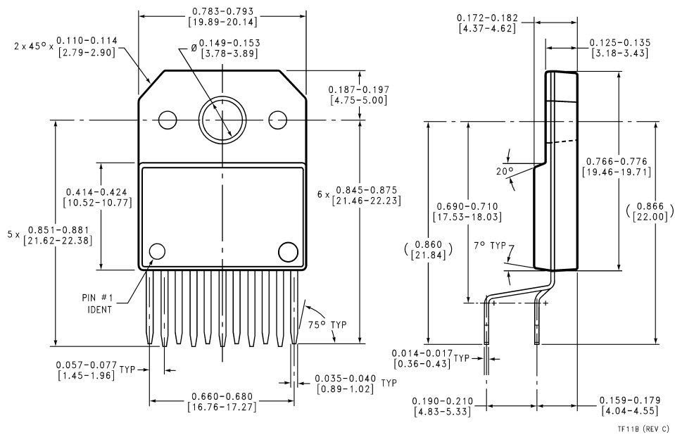
Order Number LM3886TF NS Package Number TF11B
