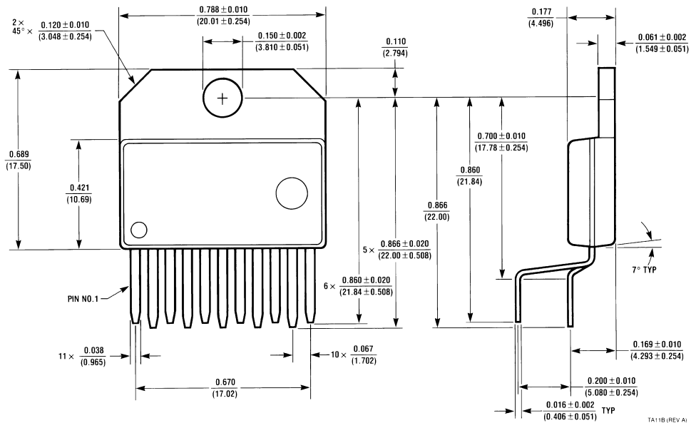
Order Number LM3886T NS Package Number TA11B
