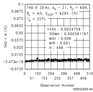
THD + N Distribution
