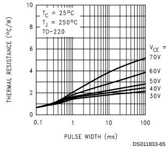
Pulse Thermal Resistance
