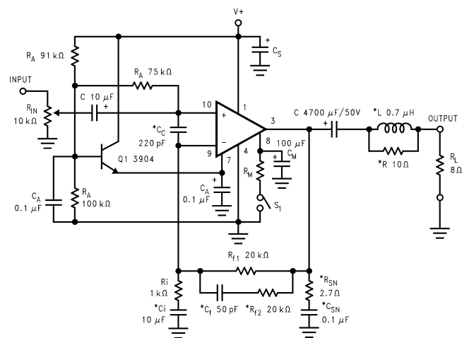
FIGURE 2. Typical Single Supply Audio Amplifier Application Circuit
