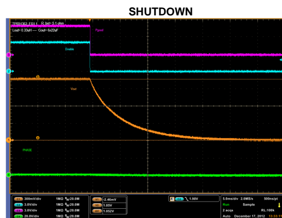
Figure 26. f = 800\text{kHz} , V_{IN} = 20\text{V} , I_{OUT} = 0\text{A}
