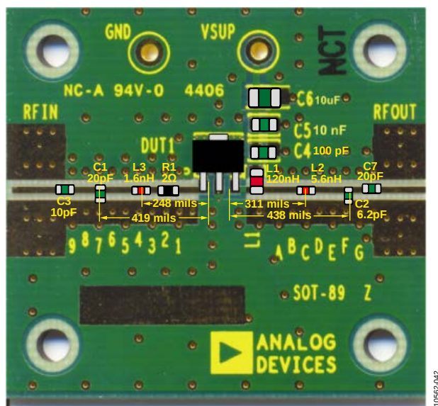
Figure 41. Evaluation Board Layout and Component Placement, 420 MHz to 494 MHz Operation
