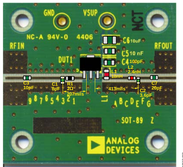
Figure 43. Evaluation Board Layout and Component Placement, 869 MHz to 961 MHz Operation
