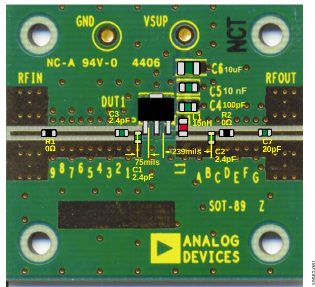
Figure 44. Evaluation Board Layout and Component Placement, 1880 MHz to 1990 MHz Operation
