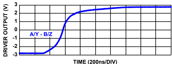
FIGURE 37. ISL32602E, ISL32603E DRIVER AND RECEIVER WAVEFORMS, LOW TO HIGH
