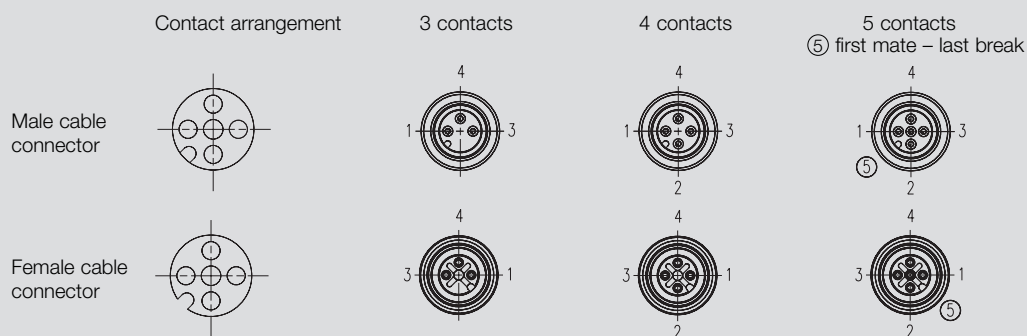
Cordset Male connector, straight / Female connector, right angled with anti-vibration coupling nut
