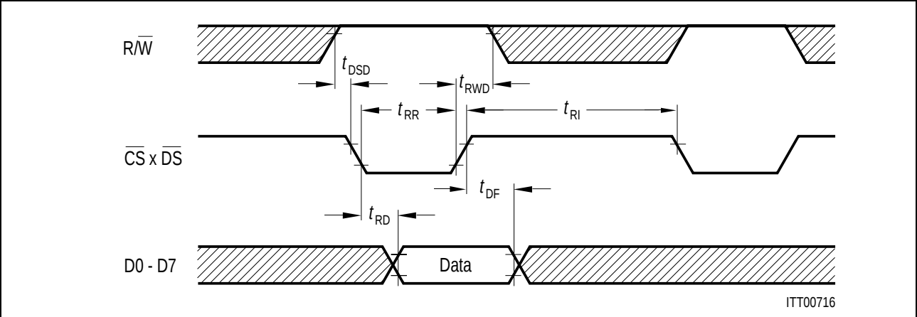
Figure 108 Motorola Read Timing
