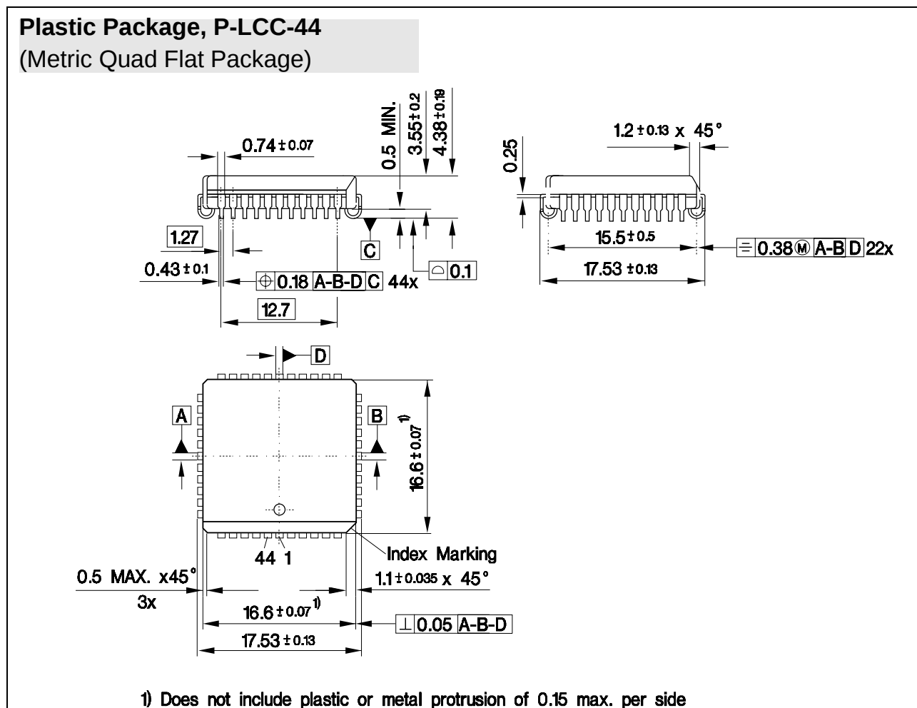
Figure 125 Package Outline for P-LCC-44
