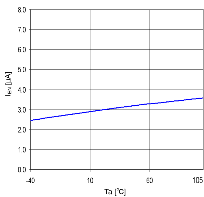
Figure 24. T_a - I_{EN}
