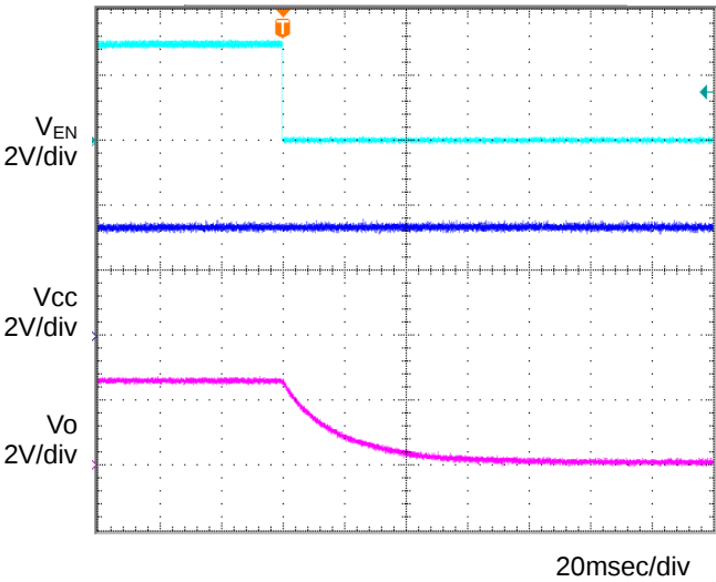
Figure 18. OFF sequence 2 C_o=1\mu F, T_a=-40^{\circ}C
