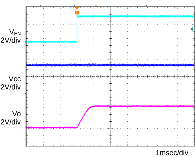
Figure 17. Input sequence 2 C_o=1\mu F, T_a=105^{\circ}C
