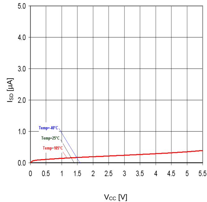
Figure 26. V_{CC} - I_{SD} ( V_{en}=0\text{V} )
