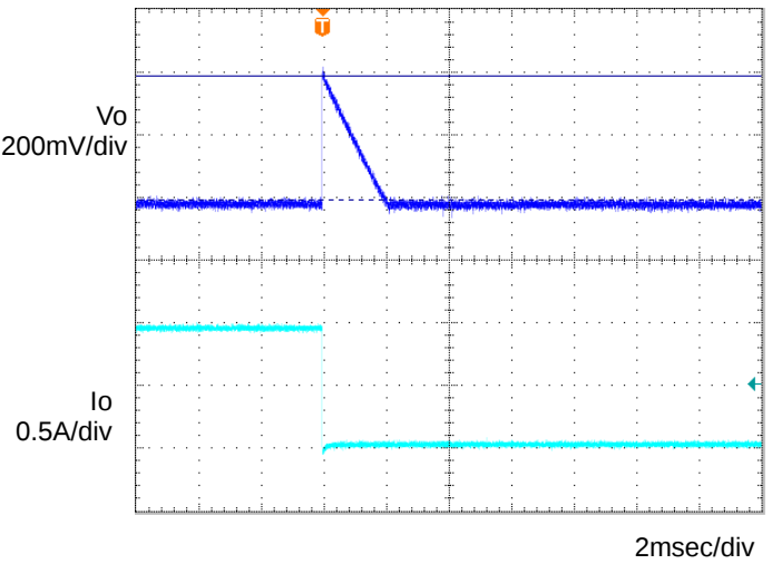
Figure 8. Transient Response (1.0→0A) C_o=1\mu F, T_a=105^{\circ}C
