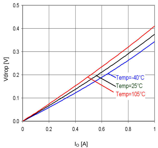
Figure 34. Minimum dropout Voltage 2 ( V_{CC}=2.4 V, T_a=25^\circ C)
