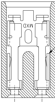
SECTION B-B
