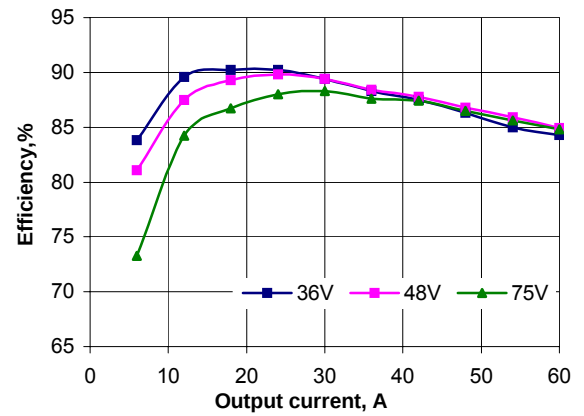
Figure 4. HHS60ZA (1.5V) Efficiency Curves
