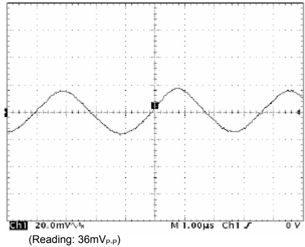
Figure 11. HHS60ZE Output Ripple Characteristics V_{in}=48V and I_{out}=3A
