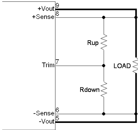
Figure 17. HHS60 Series Positive Trim Schematic
