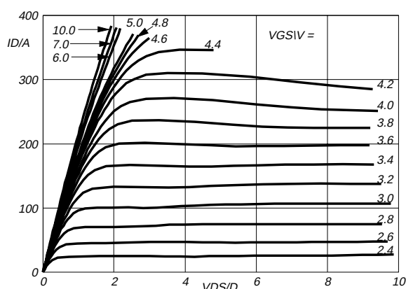
Fig.5. Typical output characteristics, T_j = 25^\circ\text{C} . I_D = f(V_{DS})
