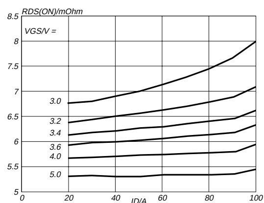
Fig.6. Typical on-state resistance, T_j = 25^\circ\text{C} . R_{DS(ON)} = f(I_D)
