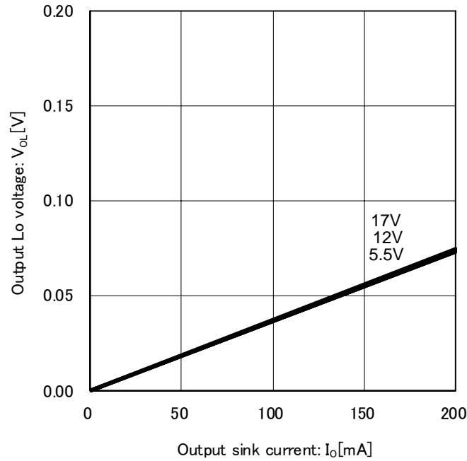
Fig.14 Output Lo voltage ( T_a=25^{\circ}C )
