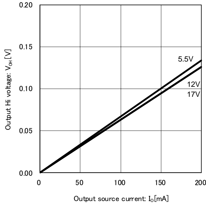
Fig.12 Output Hi voltage ( T_a=25^{\circ}C )
