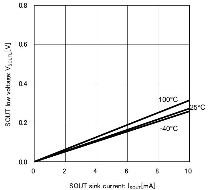
Fig.8 SOUT low voltage ( V_{CC}=12V )
