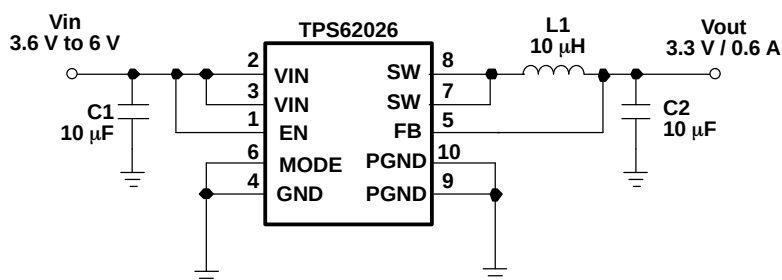
Figure 21. TPS62026 Fixed 3.3 V Output Using 10 μH inductor
