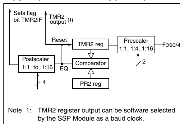
FIGURE 6-1: TIMER2 BLOCK DIAGRAM
