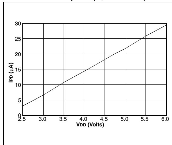
FIGURE 14-10: TYPICAL I_{PD} vs. TIMER1 ENABLED (32 kHz, RC0/RC1 = 33 pF/33 pF, RC MODE)
