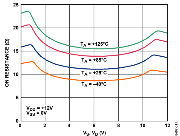
Figure 11. On Resistance as a Function of V_D ( V_S ), for Different Temperatures, 12\text{ V} Single Supply
