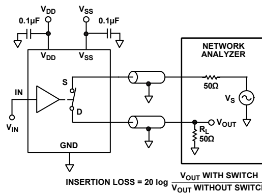
Figure 28. Insertion Loss
