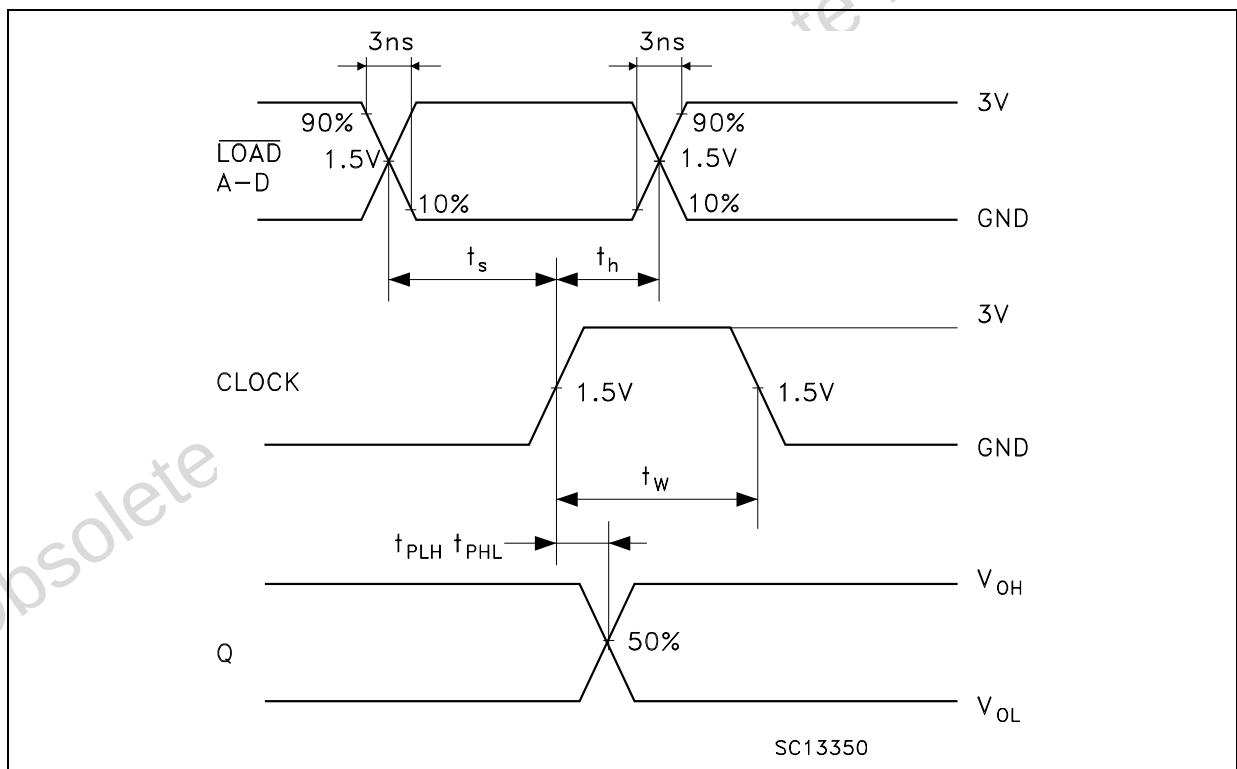
WAVEFORM 3: PROPAGATION DELAYS PRESET MODE ( f=1\text{MHz} ; 50% duty cycle)
