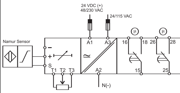
DMC01D - Namur sensor input
