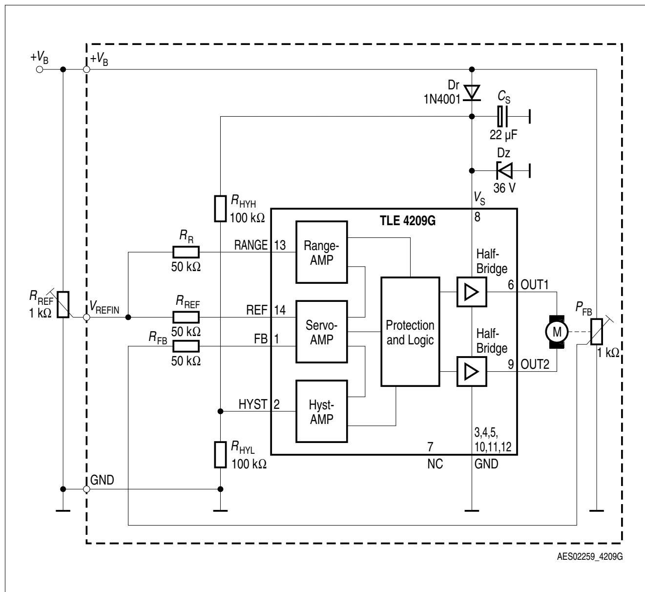
Figure 3 Application Diagram
