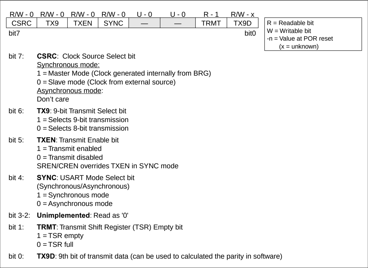
FIGURE F-10: TXSTA1 REGISTER (ADDRESS: 15h, BANK 0) TXSTA2 REGISTER (ADDRESS: 15h, BANK 4)
