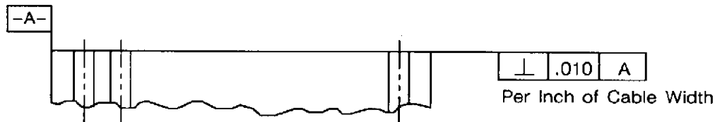
Fig. 3. Cable Edge-to-End Alignment
