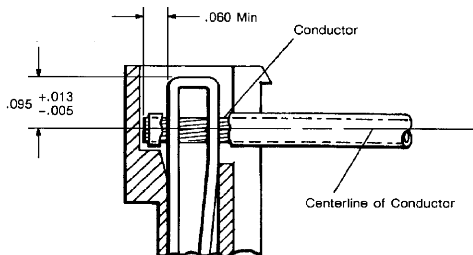
Fig. 5. Conductor Placement in Contact
