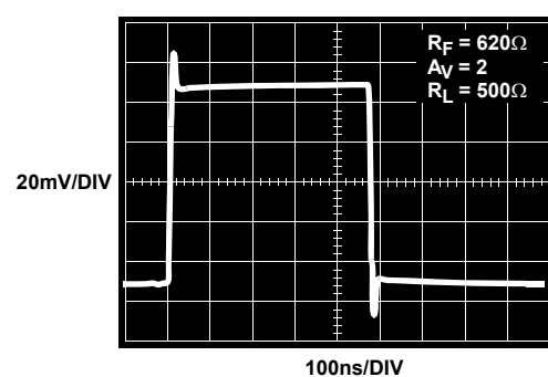
FIGURE 18. SMALL SIGNAL STEP RESPONSE ( V_S = \pm 2.5V )
