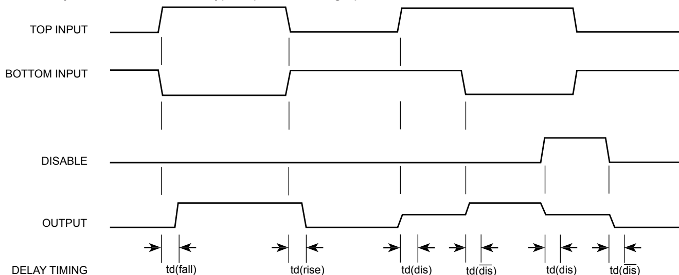
FIGURE 10. TIMING DIAGRAMS
