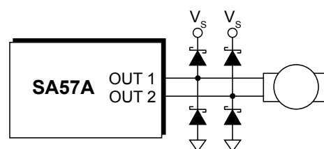
FIGURE 9. SCHOTTKY DIODES
