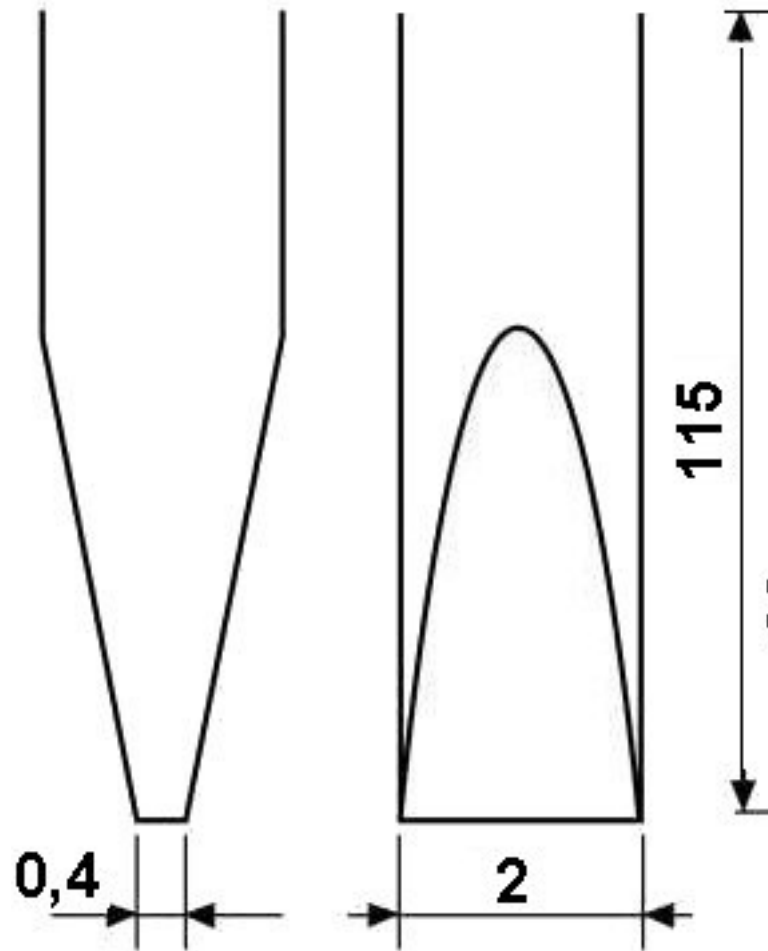
Dimensioned drawing
