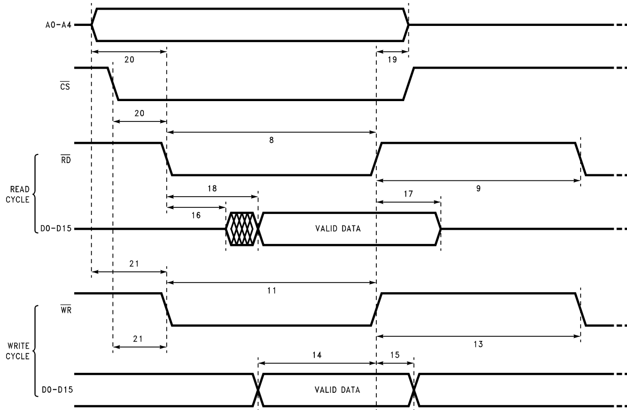
Figure 29. Non-Multiplexed Data Bus (ALE = 1)
