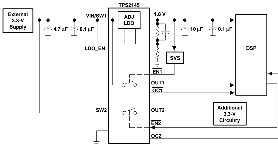
Figure 22. TPS2145 DSP With SVS Application
