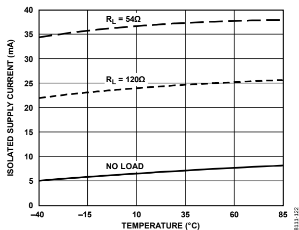
Figure 22. ADM2587E Isolated Supply Current vs. Temperature ( V_{CC} = 3.3 V, Data Rate = 500 kbps)
