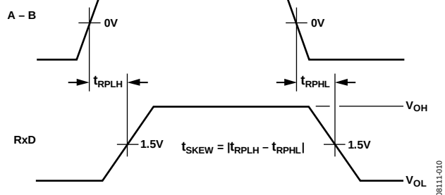
Figure 30. Receiver Propagation Delay
