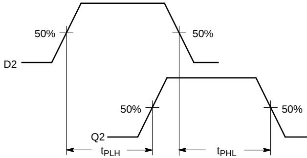
Figure 27. Single-Ended Duty Cycle Skew
