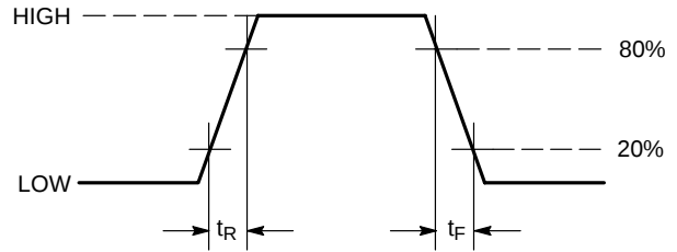
Figure 20. ECL Output Rise and Fall Times
