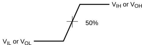
Figure 16. Single-Ended Input/Output 50% Point
