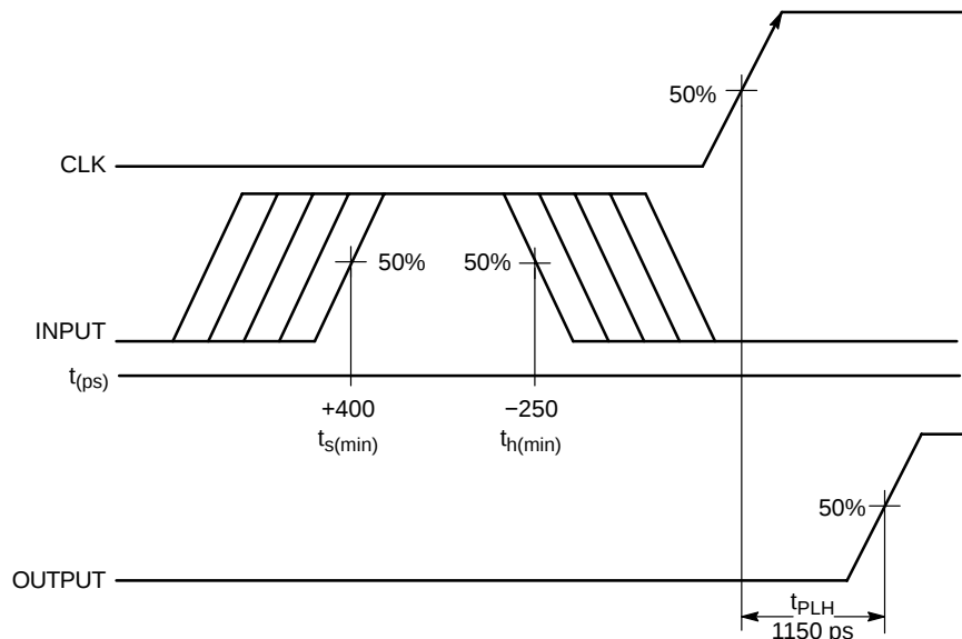
Figure 34. Positive Setup and Negative Hold Example
