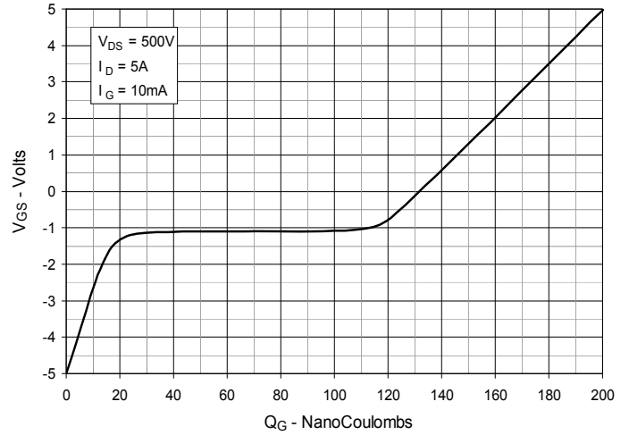
Fig. 14. Gate Charge
