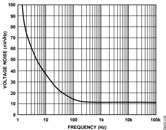
Figure 43. Voltage Noise Density vs. Frequency
