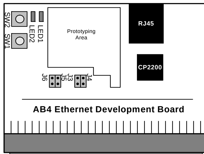
Figure 29. AB4 Ethernet Development Board
