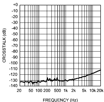
Crosstalk vs Frequency V_{CC} = 12V , V_{EE} = -12V , V_{OUT} = 3V_{RMS} A_V = 0dB , R_L = 10k\Omega
