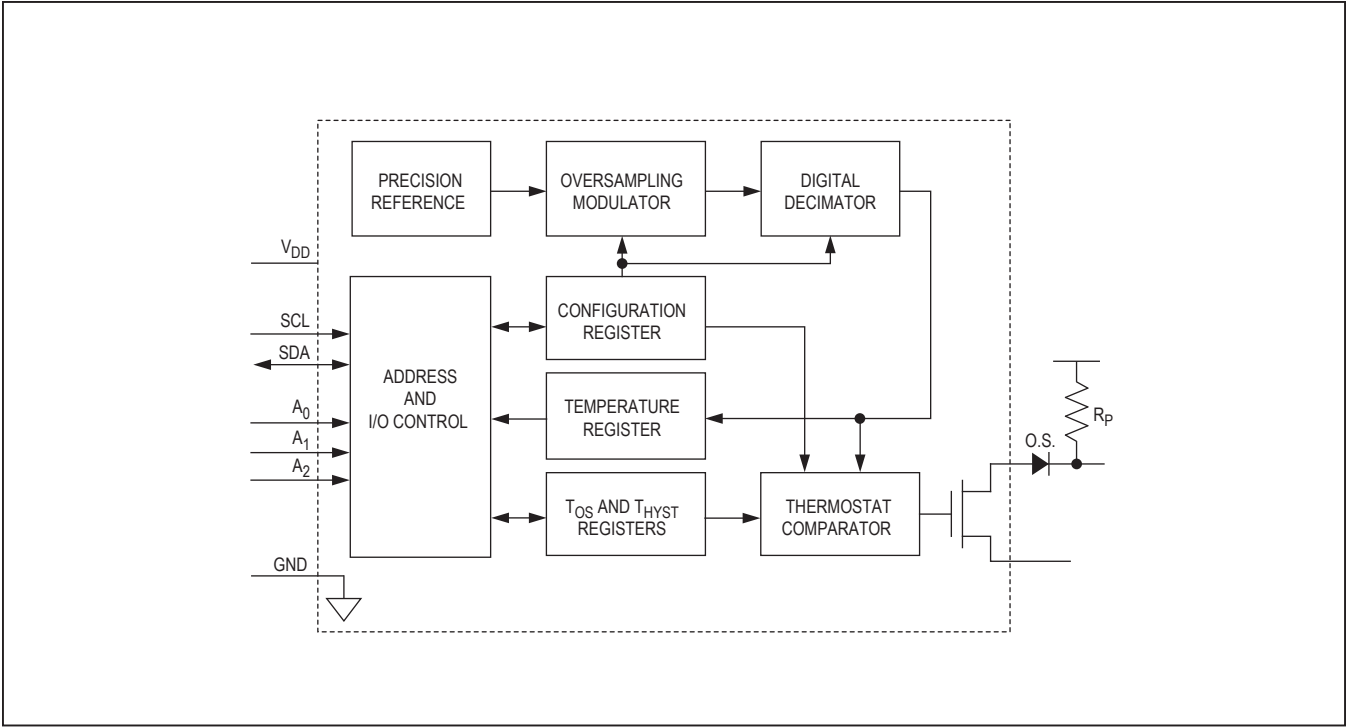
Figure 1. DS75 Functional Block Diagram
